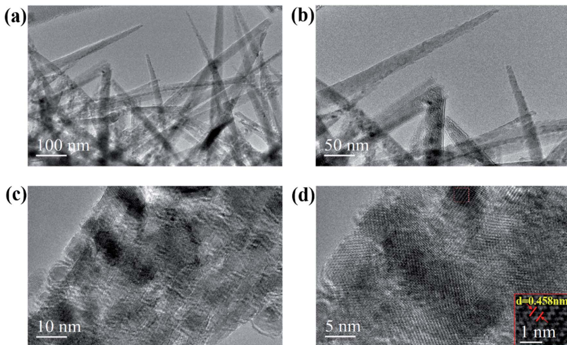
Fig. 5 (a, b) TEM and (c, d) HRTEM images of \text{NiCo}_2\text{O}_4@\text{rGO}/\text{NF} (GO 5 \text{mg L}^{-1} ).
