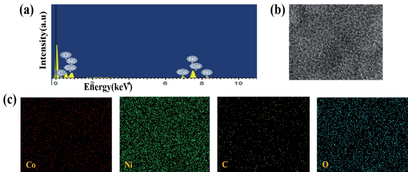
Fig. 6 (a) SEM energy dispersive spectroscopy, (b) SEM and (c) SEM element mapping of \text{NiCo}_2\text{O}_4@\text{rGO}/\text{NF} (GO 5 \text{mg L}^{-1} ).
